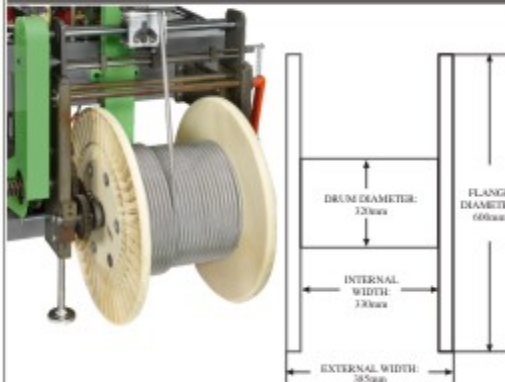
HC-OP 2 / Take Up Drum
