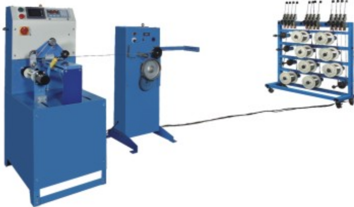
HC-01 BBS Semi-Automatic Stainless Steel Winder Set
