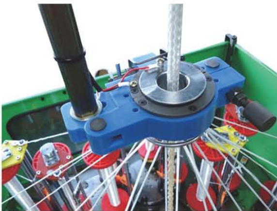
SNSR-3 Forming Eye Sensor / Openable
